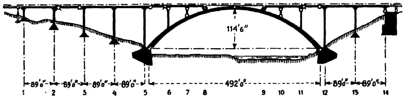
Fig. 364.—Articulation Diagram.
